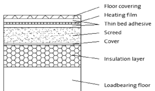
Heat insulation and installation as surface, direct heating in thin bed Adhesive.
