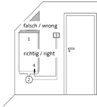
(1) Heating film (2) Transformer (3) Controller (4) Sensor
